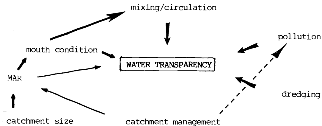
Fig.21a. Interactive diagram of the factors influencing water transparency as a component of an estuarine ecosystem.
