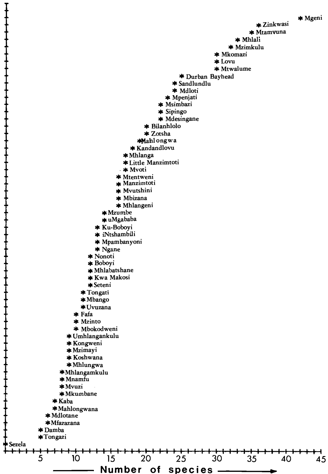
Fig.7 The relative species richness of 60 systems south of the Tugela River in Natal. To equate the relative effort expended trawl netting in each system, the total number of fish, prawn and crab species caught after three visits to each system are shown. The Vungu and Zolwane have been dropped because neither could be effectively sampled by trawling (see Appendix).
