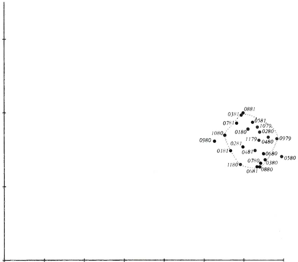
Fig.25 Temporal variation in community structure of the Mgeni Estuary after ordination of the data in Table 20 (Appendix). The core area is defined by a dotted line (0481 = April 1981, etc).
