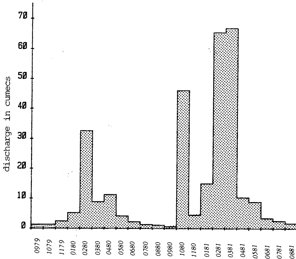
Fig.25 Flow of the Mkomazi River (from records maintained by SAICCOR, see Appendix) on those occasions the estuary was being sampled. The dates (0580 = May 1980) therefore correspond with those in Fig.24.
