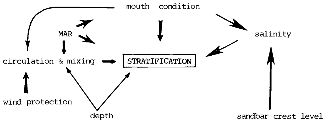
Fig. 22a. Interactive diagram of the factors influencing salinity stratification as a component of an estuarine ecosystem.
