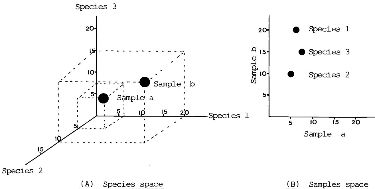
Fig.9 Spatial relationships between two samples and three species in species space (A) and samples space (B). Sample a has abundances of 6,5 and 7,5 for species 1-3 respectively; and sample b has abundances of 20,10 and 15 for species 1-3 respectively. Both A & B contain the identical information but expressed in different ways. (A) is after van Groenewoud (1965); and (B) after Gauch (1982). "Samples with similar species occupy nearby positions in species space, whereas species with similar distributions in the sample set (for example 1 & 3) occupy nearby positions in samples space" (Gauch,1982).
