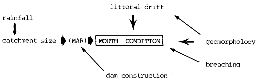
Fig.16a. Interactive diagram of the factors influencing mouth condition as a component of an estuarine ecosystem
