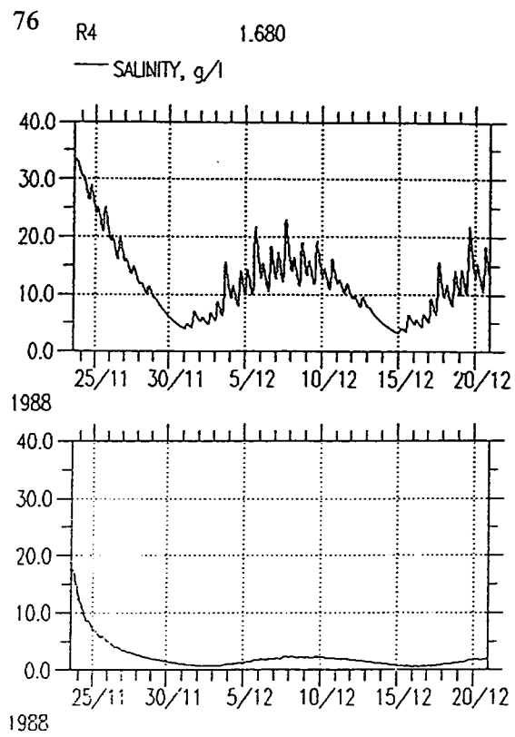
Figure 5.2 Salinities generated by Mike 11 at positions R2, R4, R6 & R8 over 28 days under the natural run-off scenario
