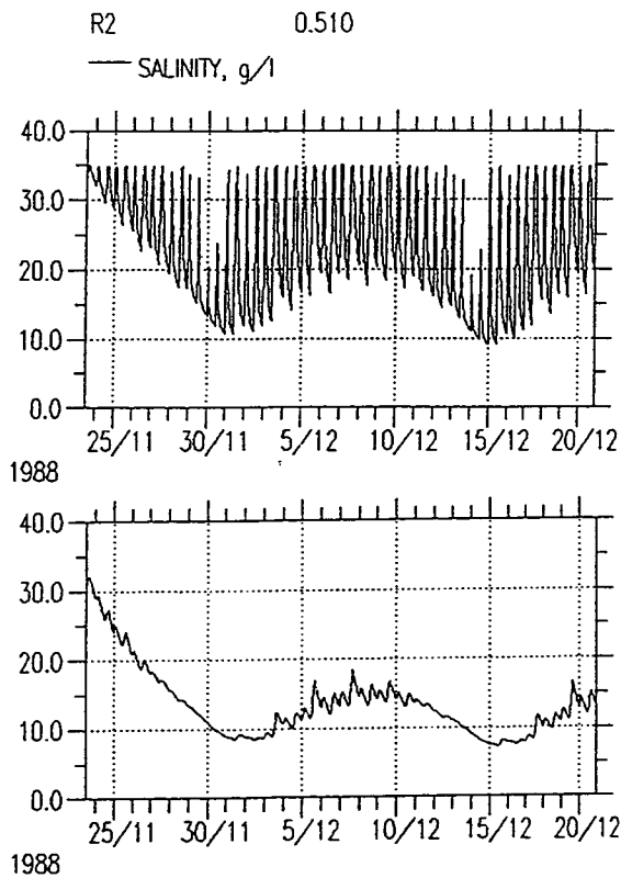
Figure 5.3 Salinities generated by Mike 11 at positions R2, R4, R6 & R8 over 28 days under the pre-dam run-off scenario
