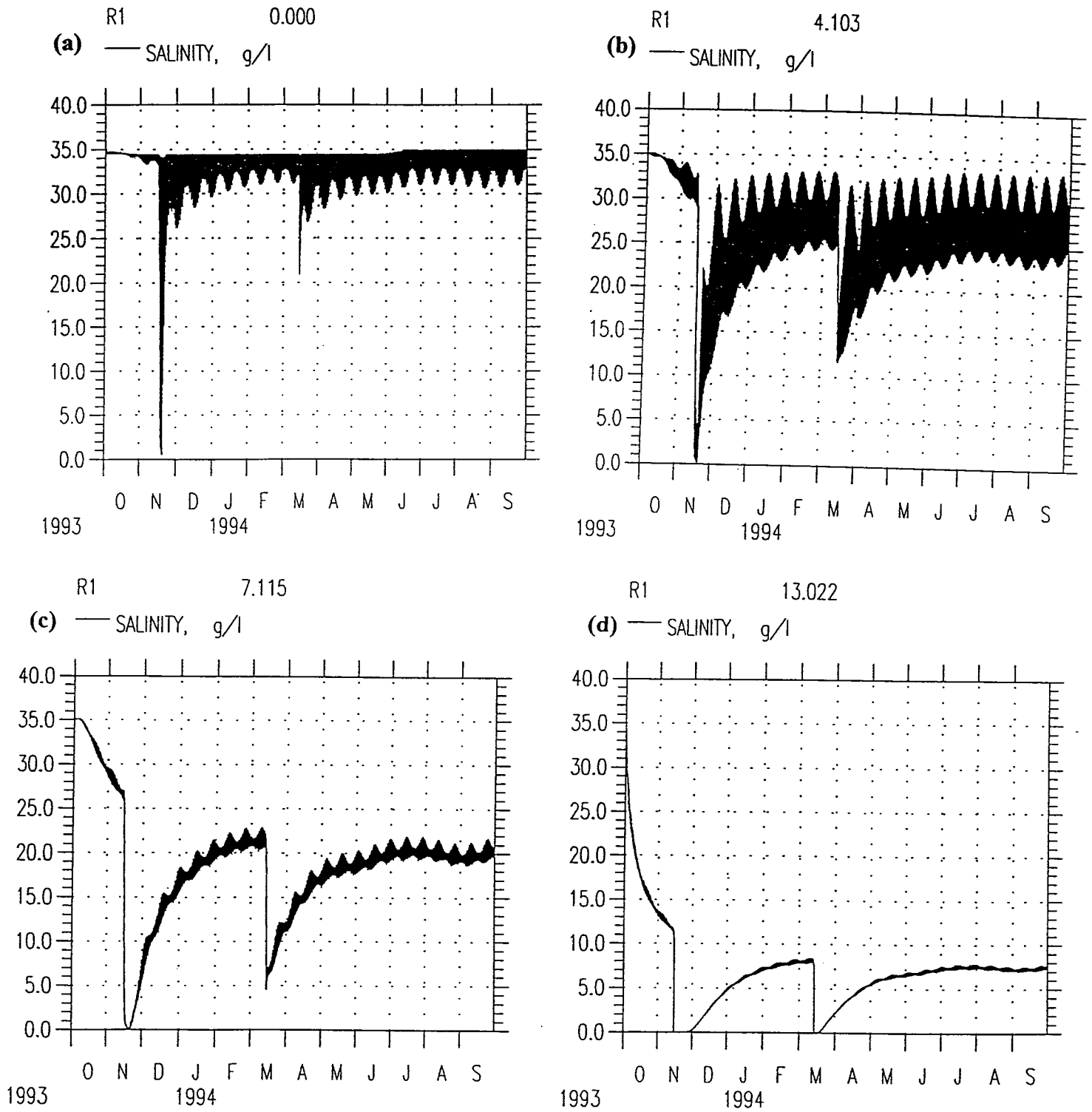
Figure 4.10 Mike 11 predictions under run-off scenario 6 at the mouth (a), in the middle reaches (b & c) and in the upper reaches (d).
