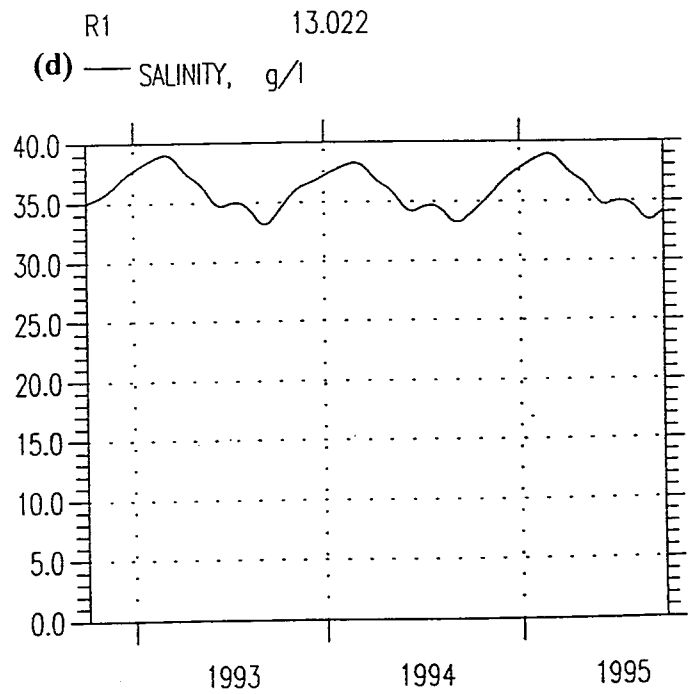
Figure 4.12 Mike 11 predictions under run-off scenario 8 at the mouth (a), in the middle reaches (b & c) and in the upper reaches (d).
