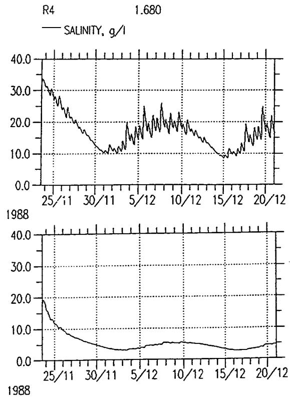
Figure 5.3 Salinities generated by Mike 11 at positions R2, R4, R6 & R8 over 28 days under the pre-dam run-off scenario
