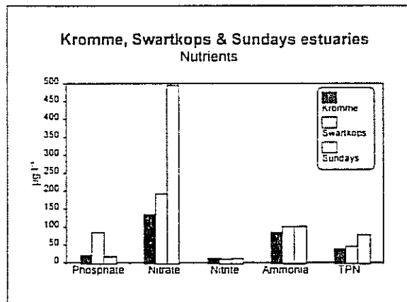
Fig. 4.2.: Mean estuarine nutrient concentrations in the Kromme, Swartkops and Sundays estuaries. Bars denote mean values for the whole study period.
