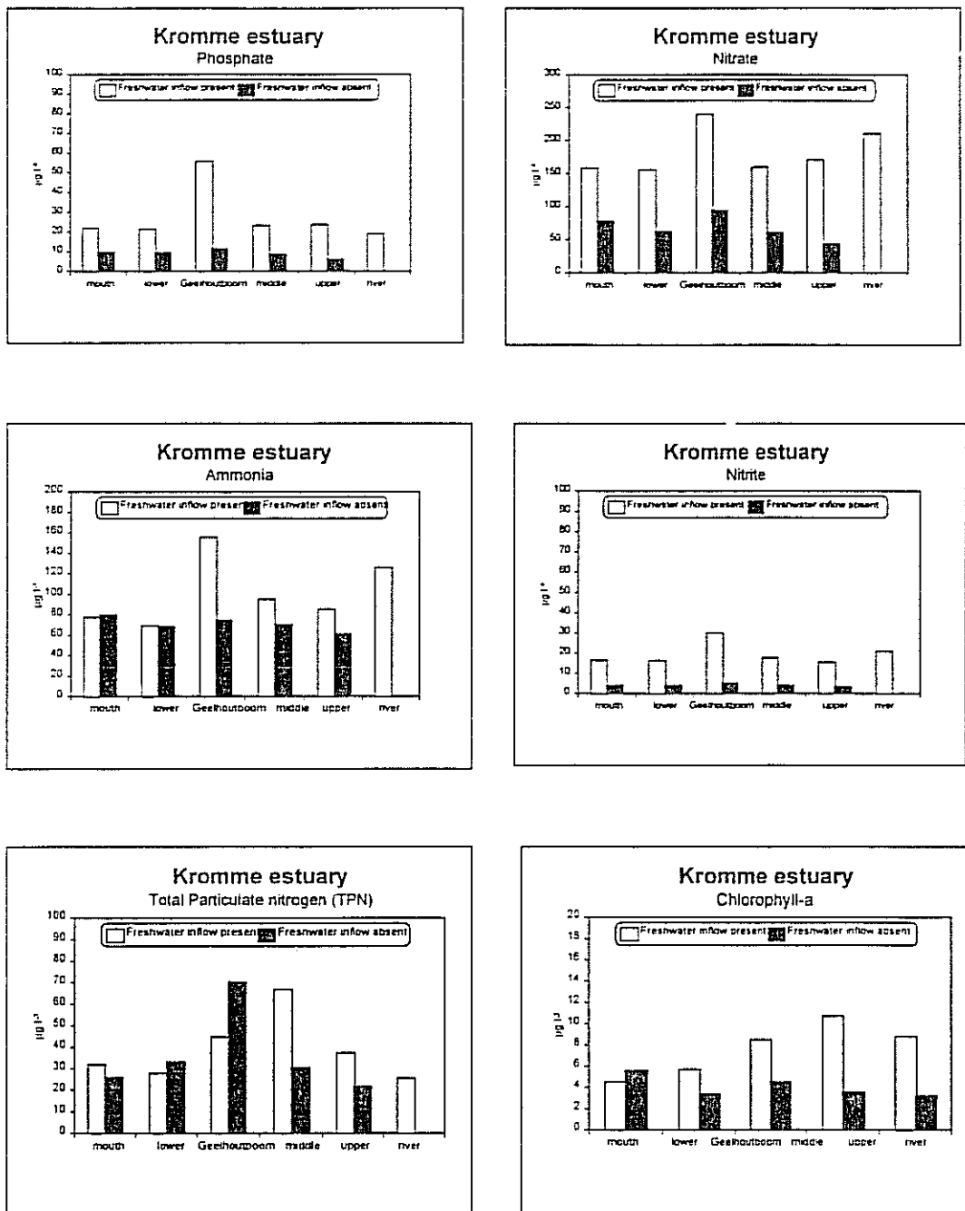
Fig. 4.4: Nutrient and chlorophyll-a concentrations for the Kromme and Geelhoutboom estuaries for periods of occurrence and non-occurrence of freshwater inflow. Bars denote mean values for the respective periods of present/absent freshwater inflow.
