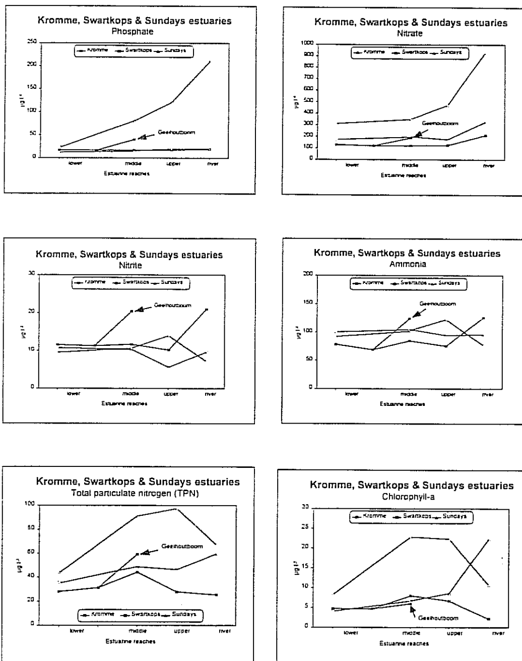
Fig. 4.3: Longitudinal gradients for several nutrients and chlorophyll-a in the Kromme, Swartkops and Sundays estuaries. Datapoints are mean values for the whole study period.
