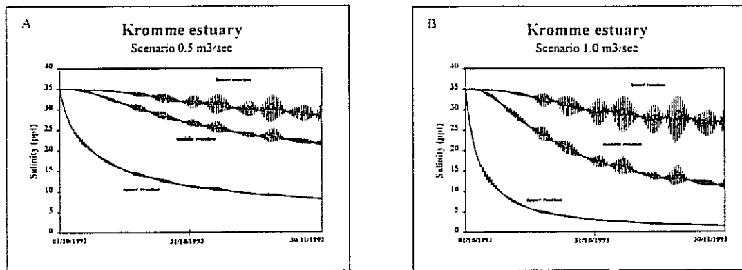
Fig. 3.9: Salinities at the lower, middle and upper reaches of the Kromme estuary as a result of two freshwater inflow scenarios ( 0.5 \text{ m}^3\text{-sec}^{-1} (A); 1 \text{ m}^3\text{-sec}^{-1} (B)) simulated by the Mike 11 hydrodynamic model over a period of 2 months.
