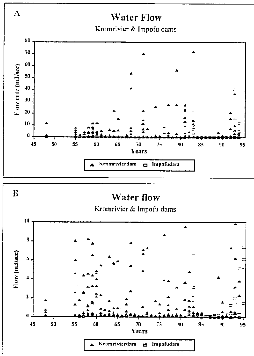
Fig. 3.13: Water flow at the Kromrivier and Impofu dam. Datapoints are monthly flow rates, which were supplied by the Department of Water Affairs (Pretoria). B is an enlargement of A.
