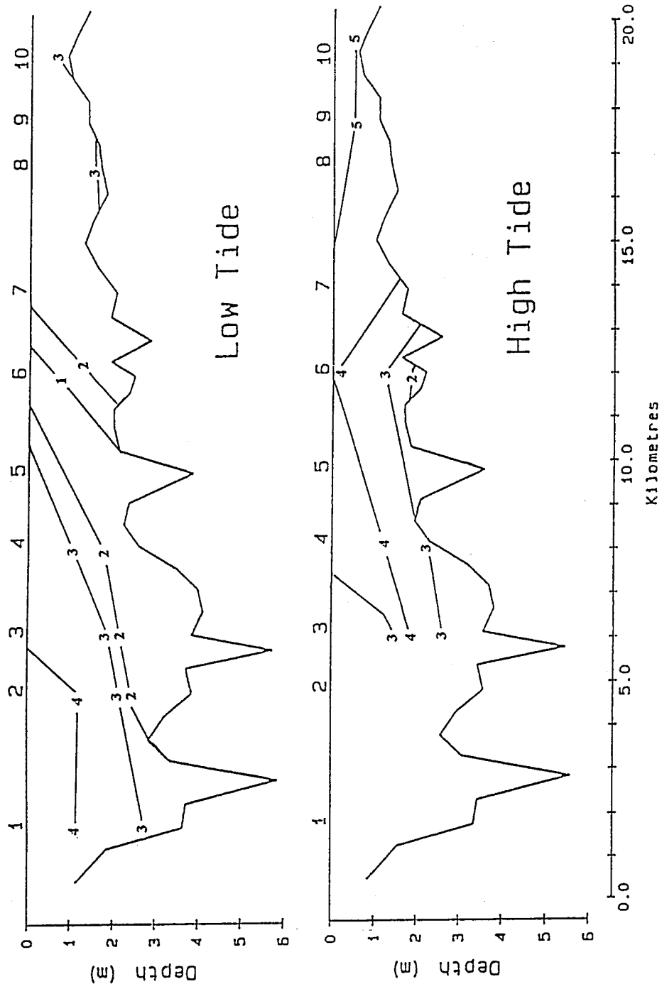
Figure 4.24 Dissolved oxygen ( \text{mg l}^{-1} ) profiles at low and high tide on 16 June 1993.
