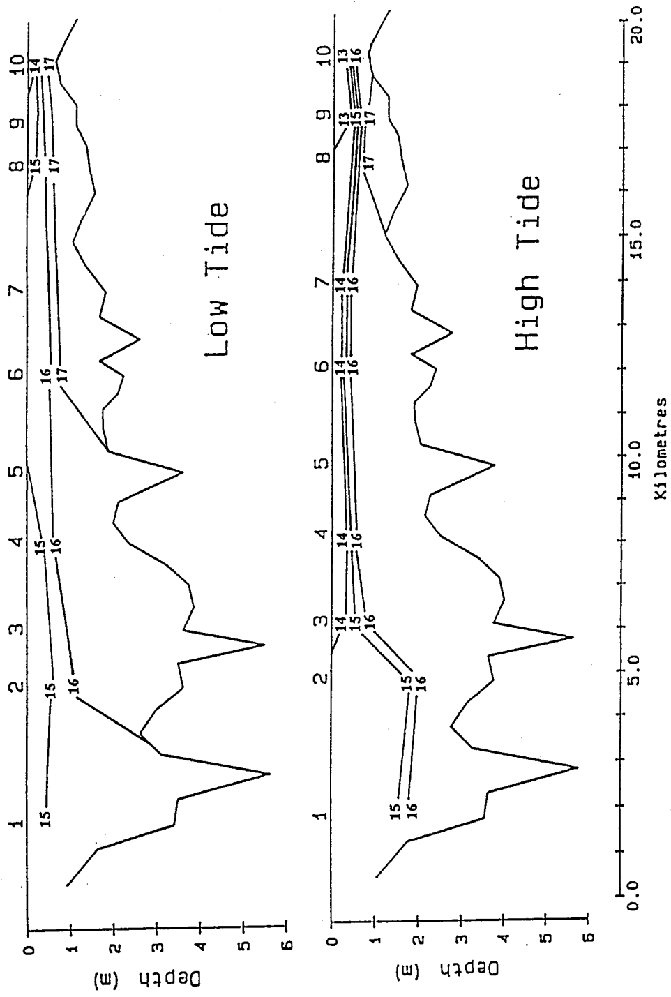
Figure 4.17 Temperature ( ^{\circ}\text{C} ) profiles at low and high tide on 7 June 1993.
