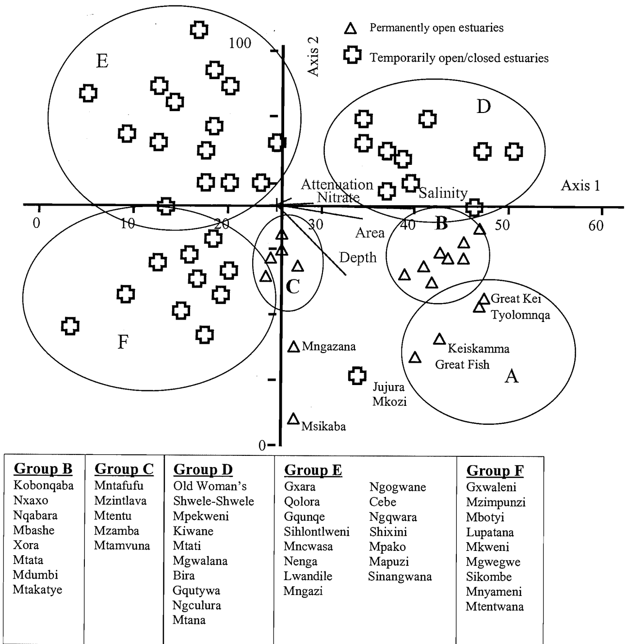
Figure 6.2 CCA ordination of estuaries based on plant species presence/absence in the Ciskei and Transkei regions. Spatial separation of the estuaries in relation to environmental variables and the distribution of plants species are shown. Environmental variables include water column depth, average salinity and secchi depth.
