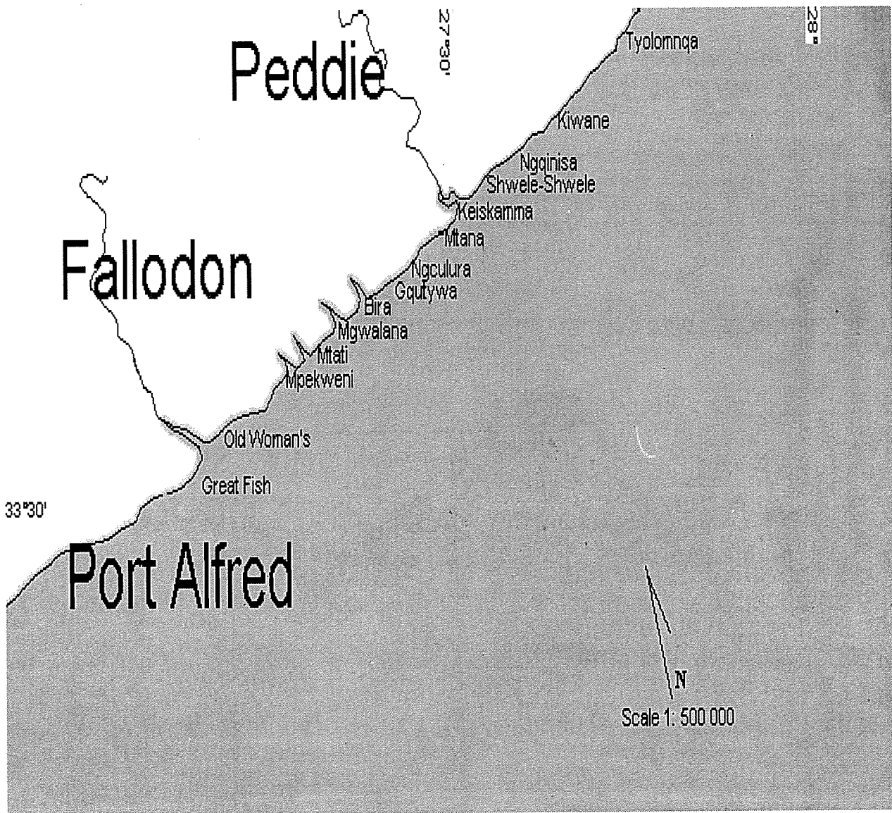
Figure 2.1: The Ciskei study region, with sixteen estuaries. The Great Fish, Keiskamma and Tyolomnqa Estuaries are the only permanently open estuaries.
