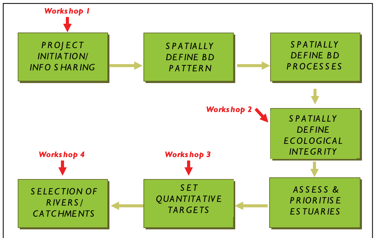
Figure 1: Step-wise planning framework adopted The framework is based upon the fundamental principles of systematic conservation planning, and includes a series of workshops at key milestones in which workshop participants are provided the opportunity to influence both the approach and the outcomes.
