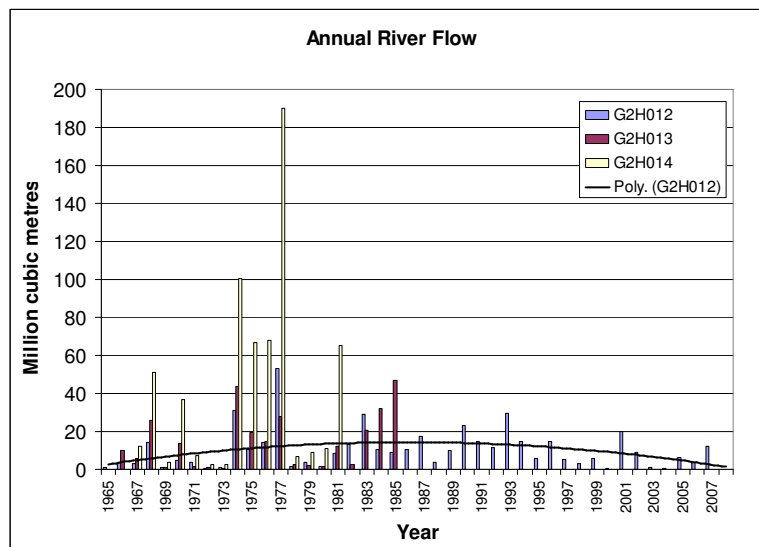
Figure 5. Annual flow data for the 3 gauging stations with polynomial fit to G2H012.
