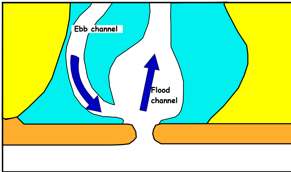
Figure 1.2. Typical configuration of ebb and flood tidal channels in the mouth region of an estuary (Huizinga and van Niekerk 2005).
