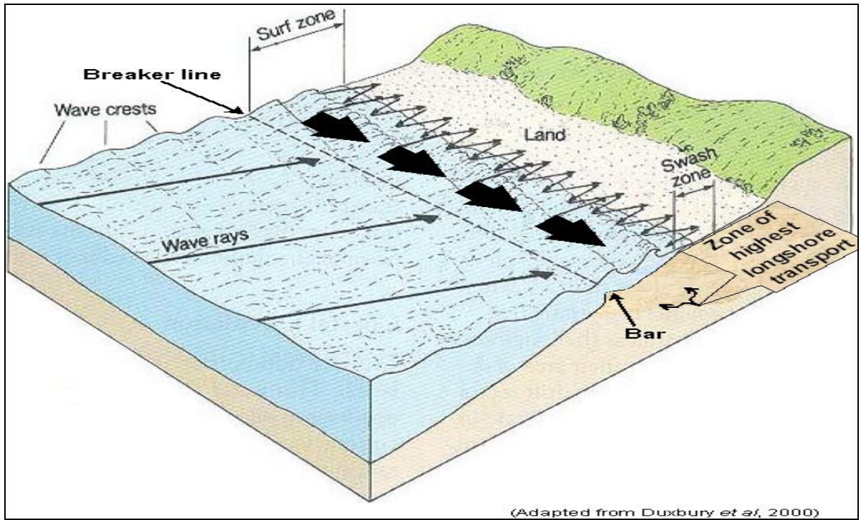
Figure 2.2. Schematic diagram showing longshore transport.
