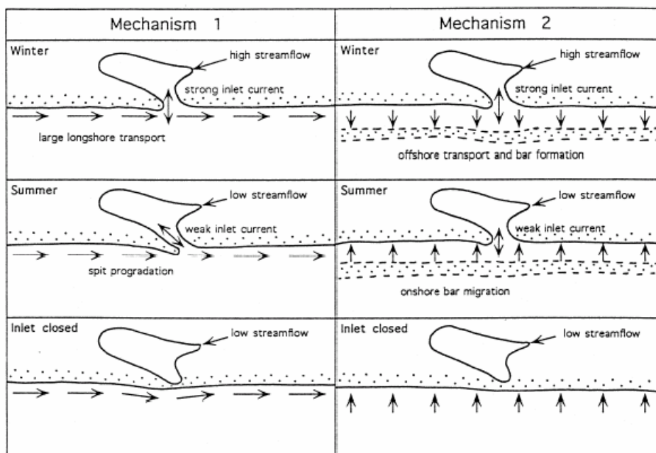
Figure 2.1 Schematic depiction of inlet closure by longshore processes and cross-shore processes.
